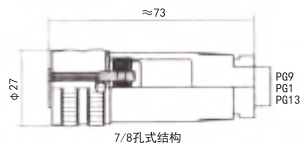
FIG 1 Female Straight w/ Internal Threads
